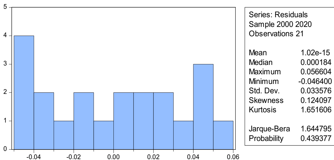
Figure 2: Normality test
