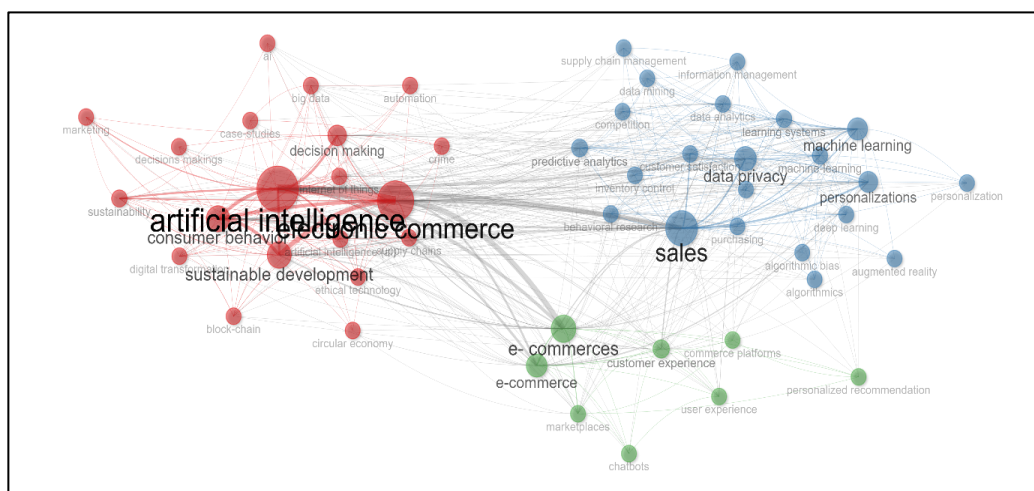
Figure 9: Co-occurrence Network
